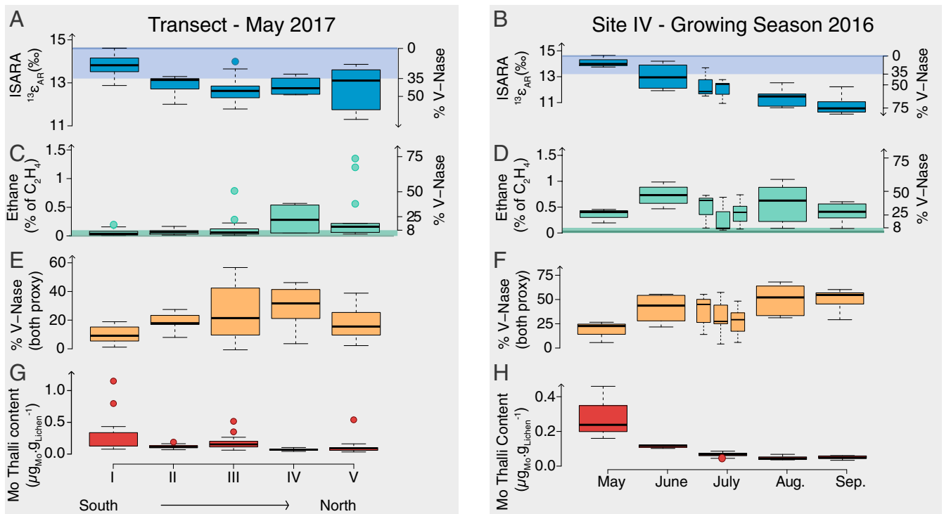
Fig. 2. Alternative V-Nase activity and Mo thalli content along the south–north transect described in Fig. 1 ( A, C, E, and G ) and growing season at site IV ( B, D, F, and H ). The boxplots show the ISARA carbon isotopic fractionations ( A and B ), ethane productions ( C and D ), and contributions of alternative V-Nase to the total BNF activity calculated as the average of both methods when available ( E and F ). Molybdenum contents of the thalli are shown for comparison ( G and H ). In A–D , the right axis represents the estimated contribution of V-Nase to BNF (note the direction of axis). Filled symbols represent values outside the whiskers, i.e., 1.5 interquartile range over the upper quartile or below the lower quartile. When filled symbols are absent, the whiskers represent the full range of the data. The horizontal colored boxes in A–D show the range of Mo-only signal for each proxy (ethane, <0.1\% of \text{C}_2\text{H}_4 ; ISARA, ^{13}\epsilon_{\text{AR}} > 13.2\text{‰} ).
